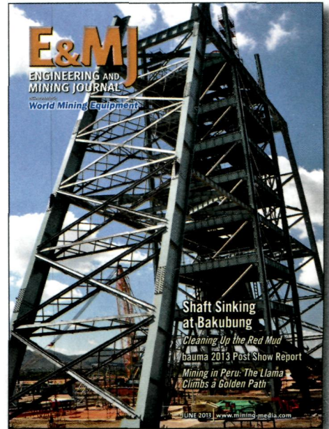
The Bakubung platinum mine plans to raise 230,000 metric tons per month (mt/m) of ore to the surface from a 1,000-m deep main shaft. The superstructure (on the cover) stands 86-m high and holds 1,860-mt of headgear.
