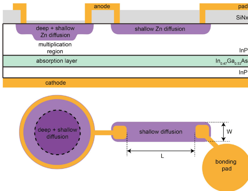
Schematic representation of a SPAD connected to a diffused quenching resistor: cross-section (top) and top view (bottom). The connection between the SPAD anode and the resistor can be made by a metal strip (as shown here) or by just extending the SPAD shallow diffusion. The SPAD active area is highlighted by the dashed line. (Sanzaro et al, Article #4500207).
