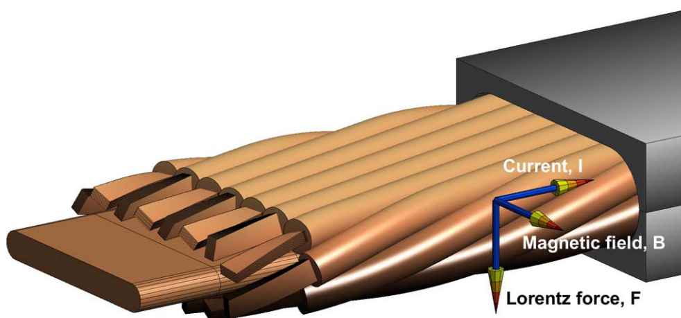
Figure 11 from “Design Optimization of Round Strands Made by Twisted Stacks of HTS Tapes,” by Bykovsky et al. , 4201207.
