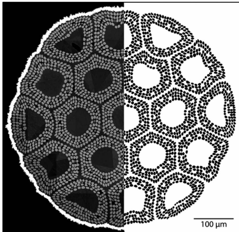
Figure 2 from “Fracture Strength Distribution of Individual \text{Nb}_3\text{Sn} Filaments,” by Dylla et al. , 6001907.
