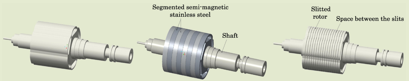
IPM rotor with (left) unmodified solid rotor, (middle) axially segmented rotor settled on stainless steel shaft, and (right) circumferentially slitted/milled solid rotor. (Taken from “High-Speed Solid Rotor Permanent Magnet Machines: Concept and Design” by P. Arumugan et al. , pp. 391–400.)
