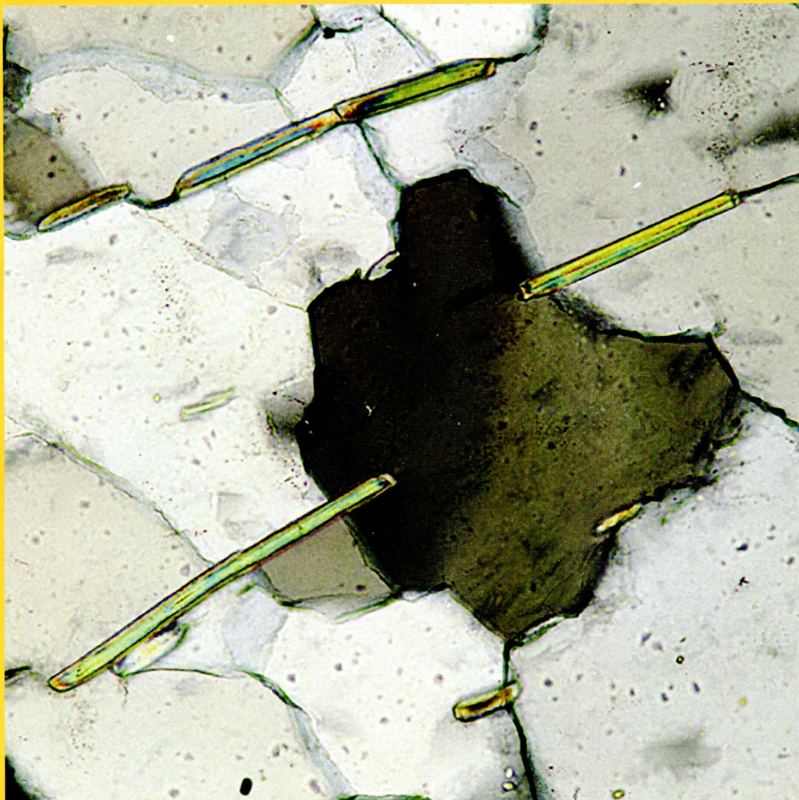
Photomicrograph (crossed nicols) of Detrital Muscovite Mica That Links Quartz Grains in Flexible Sandstone (see page 5A)
