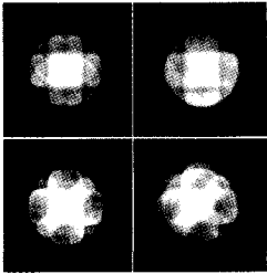
Simulated (left) and experimental (right) position-averaged convergent beam electron diffraction patterns of projections from two different GdTiO 3 orientations. [J. Y. Zhang et al. , Phys. Rev. Lett. 110 , 256401 (2013)]
