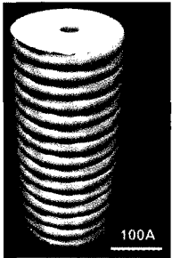
Simulated real-space image of a portion of a tobacco mosaic virus expected from x-ray free electron laser (XFEL) diffraction patterns from random orientations of the virus. Selected for a Synopsis. [Poon, H.-C. et al. , Phys. Rev. Lett. 110 , 265505 (2013)]
