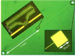
Optical microscope image of a fluxonium qubit inductively coupled to an antenna. [U. Vool et al. , Phys. Rev. Lett. 113 , 247001 (2014)]
