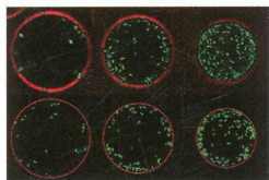
(Top) Confocal images and (bottom) simulations of emulsion drops filling with Escherichia coli bacteria. [I. D. Vladescu et al. , Phys. Rev. Lett. 113 , 268101 (2014)]
