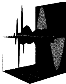
Position component of Wigner function flow: the figure shows its contours (floor) and projections along time (blue) and momentum (rose). Selected for an Editors' Suggestion. [Ole Steuernagel, Dimitris Kakofengitis and Georg Ritter, Phys. Rev. Lett. 110 , 030401 (2013)]
