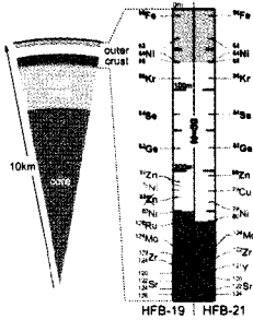
Depth profile of a neutron star. Red type indicates how the predicted composition changes on the basis of a precision mass measurement of the neutron-rich isotope {}^{82}\text{Zn} . Selected for a Synopsis in Physics. [R. N. Wolf et al. Phys. Rev. Lett. 110 , 041101 (2013)]
