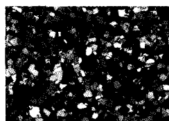
Nanocrystalline grains in Pd thin films imaged with high resolution automated crystal orientation and phase mapping combined with transmission electron microscopy. [Jochen Lohmiller et al. , Phys. Rev. Lett. 110 , 066101 (2013)] (Image by A. Kobler and C. Kübel, KIT).
