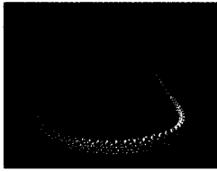
Typical snapshot from molecular dynamics simulations of the formation of a one-micron-long S-shaped carbon nanotube structure (serpentine) on a stepped graphite substrate. [L. D. Machado et al. , Phys. Rev. Lett. 110 , 105502 (2013)]
