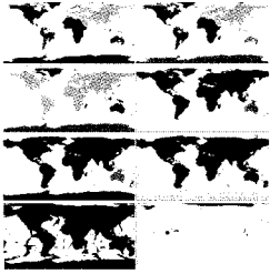
Percolation description of the Earth's global topography showing continental (oceanic) aggregation with decreasing sea level from top left to bottom right (right). [Abbas Ali Saberi, Phys. Rev. Lett. 110 , 178501 (2013)]
