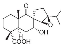
Holophyllin A (1)
