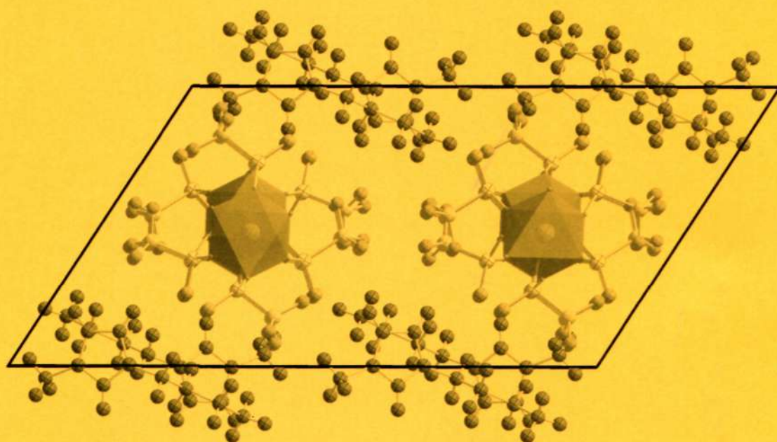
Unit cell of [BMIm][Fe(OTf) 3 ]
