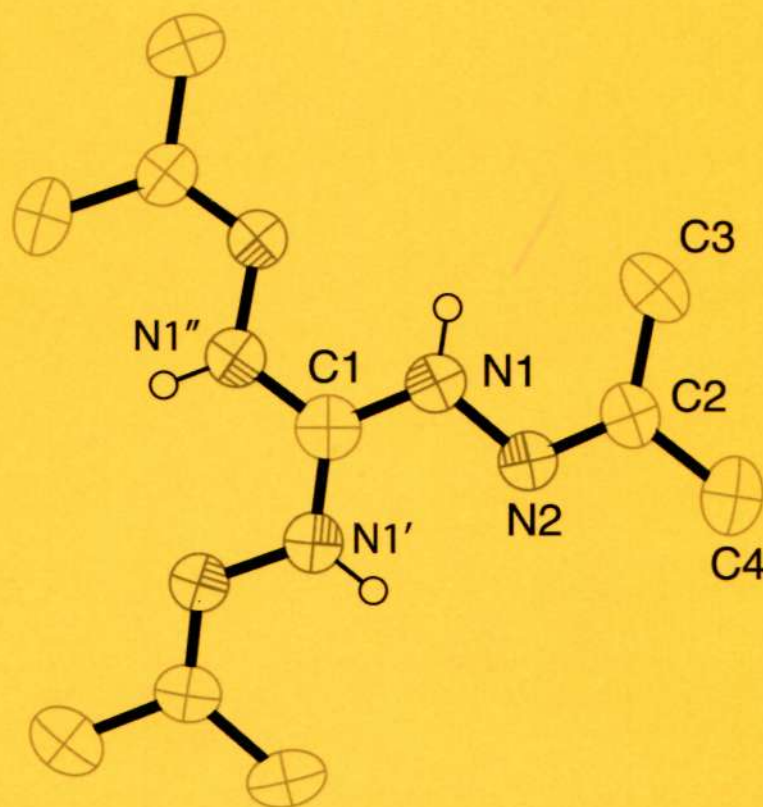
Structure of N,N',N'' -tris(propan-2-iminyl)guanidine
