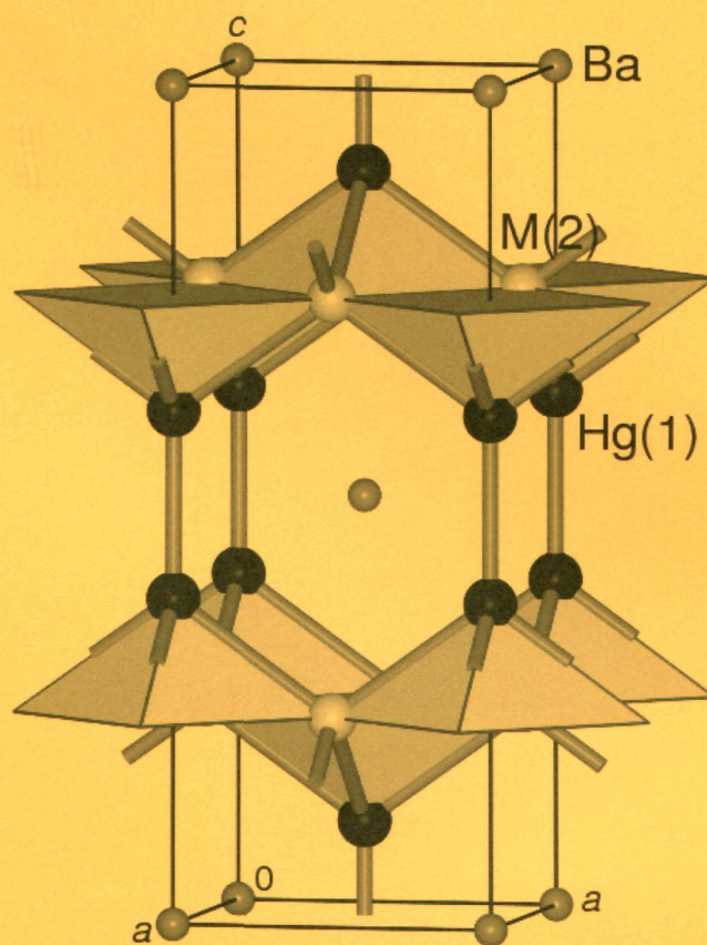
Crystal structure of \text{BaIn}_{1.7}\text{Hg}_{2.3}
