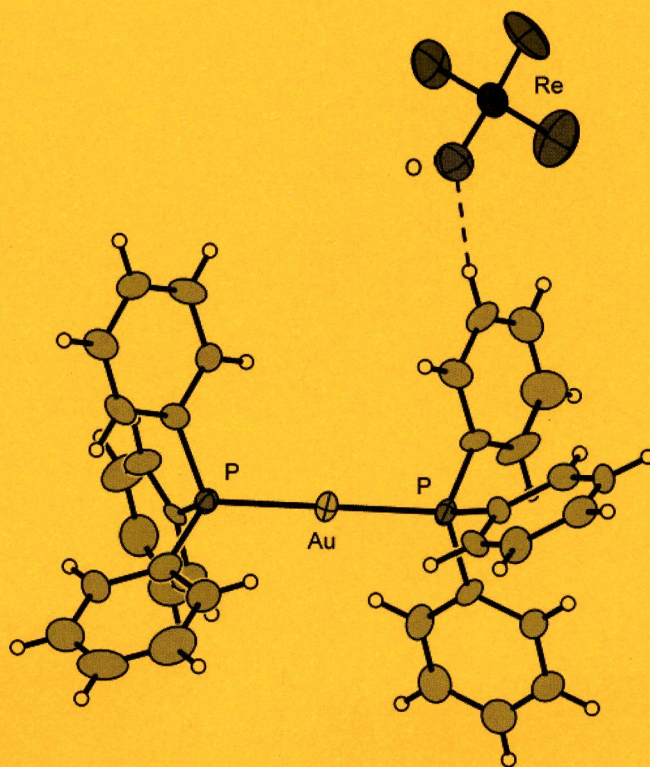
Bis(triphenylphosphine)gold(I) Perrhenate
