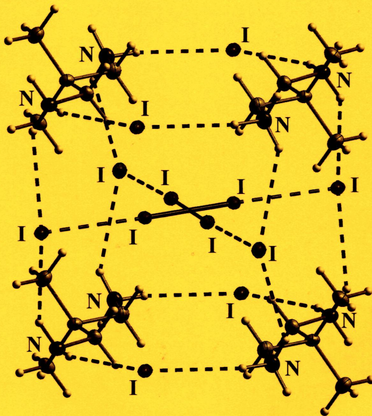
Cube-shaped building unit in (C_5H_{16}N_2)_2I_4 \cdot I_2
